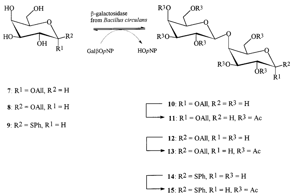
Scheme 2. Galactosylation of galactose derivatives with \beta -galactosidase from Bacillus circulans
