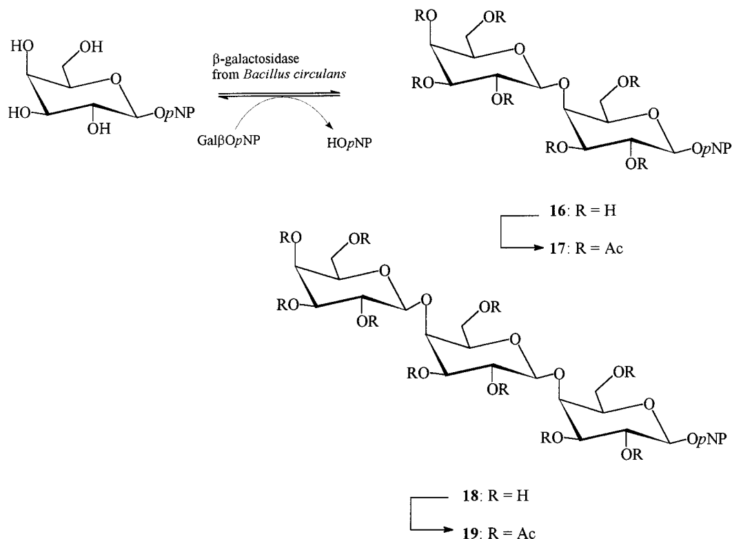
Scheme 3. Galactosylation with \beta -galactosidase from Bacillus circulans using Gal \beta OpNP as both donor and acceptor substrate
