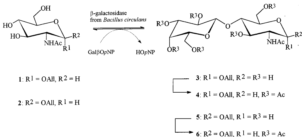
Scheme 1. Galactosylation of GlcNAc derivatives with \beta -galactosidase from Bacillus circulans
